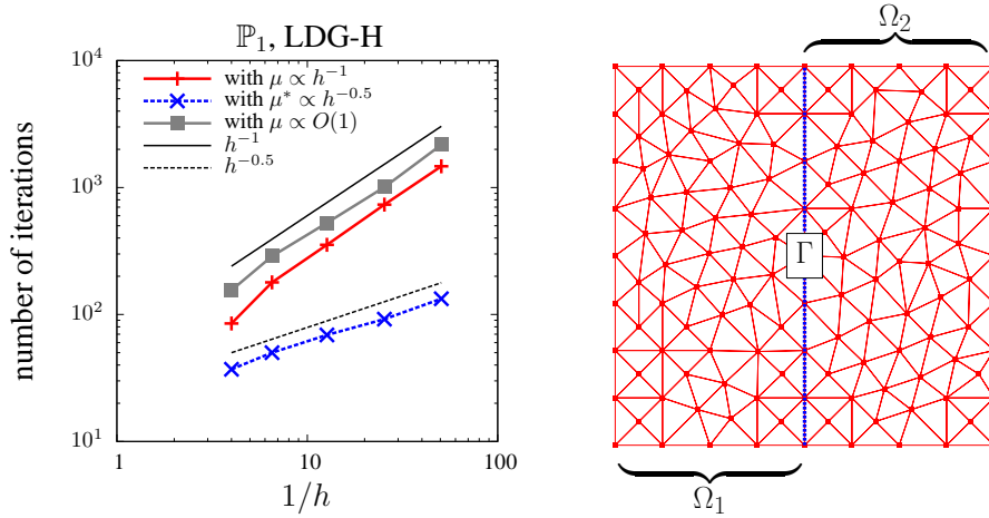
Fig. 1 (left) asymptotic number of iterations required by the non-overlapping Schwarz method using LDG-H. (right) unstructured mesh with the interface \Gamma^I = \{0.5\} \times (0, 1) .
